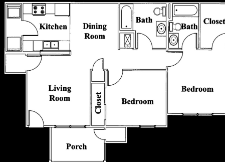
Two Bedroom Floor Plan 942-1020 sq. ft.
