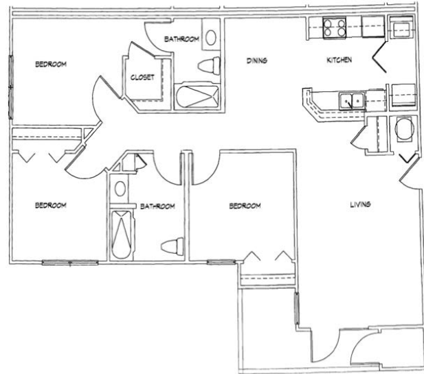
Three Bedroom / Two Bath 1140 Sq. Ft.
