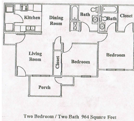
Two Bedroom / Two Bath 964 Square Feet
